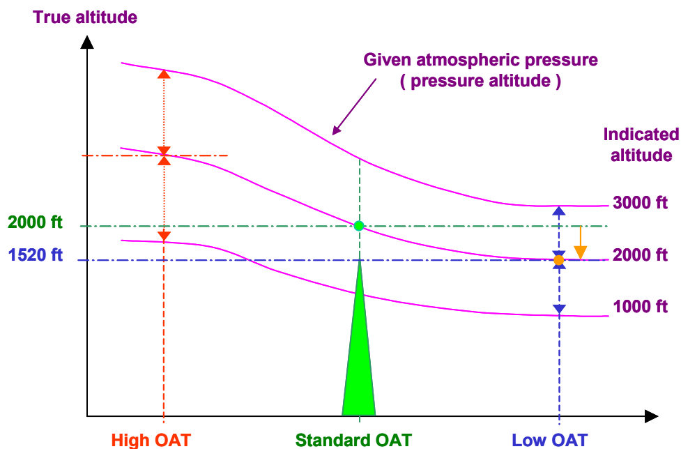
Figure 4 Effect of OAT on True Altitude
